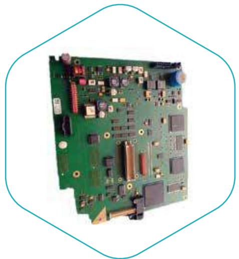
Supporting Board for MP70
